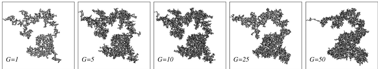
FIG. 13. Typical configurations of invaded clusters at different generations G and L=256 . The random number p_i is drawn from a uniform distribution of probabilities in the interval [p^*] for p^*=0.9 .
